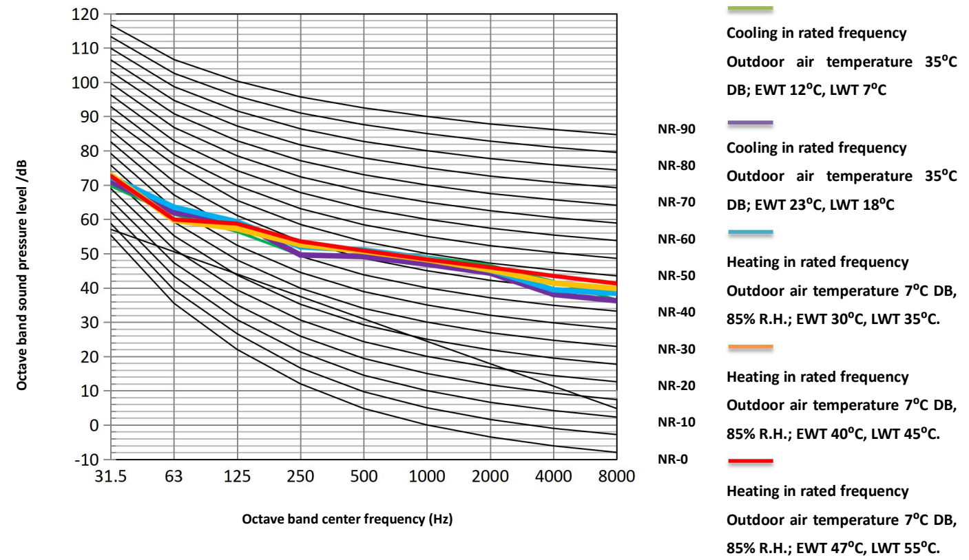
MHC-V16W/D2RN8-B2(E30/ER90) octave band levels
