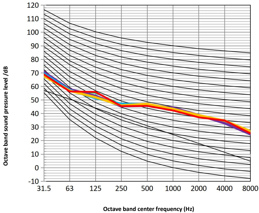
MHC-V8W/D2N8-B2(E30/ER90) octave band levels
