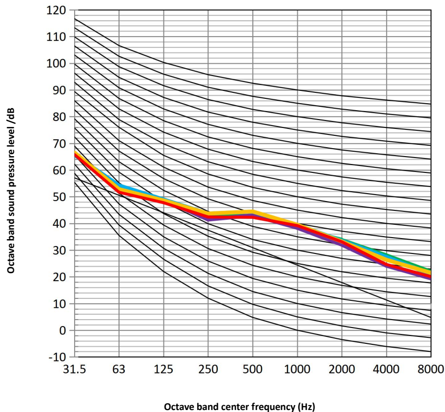
MHC-V6W/D2N8-B2(E30) octave band levels
