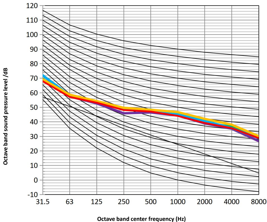
MHC-V10W/D2N8-B2(E30/ER90) octave band levels
